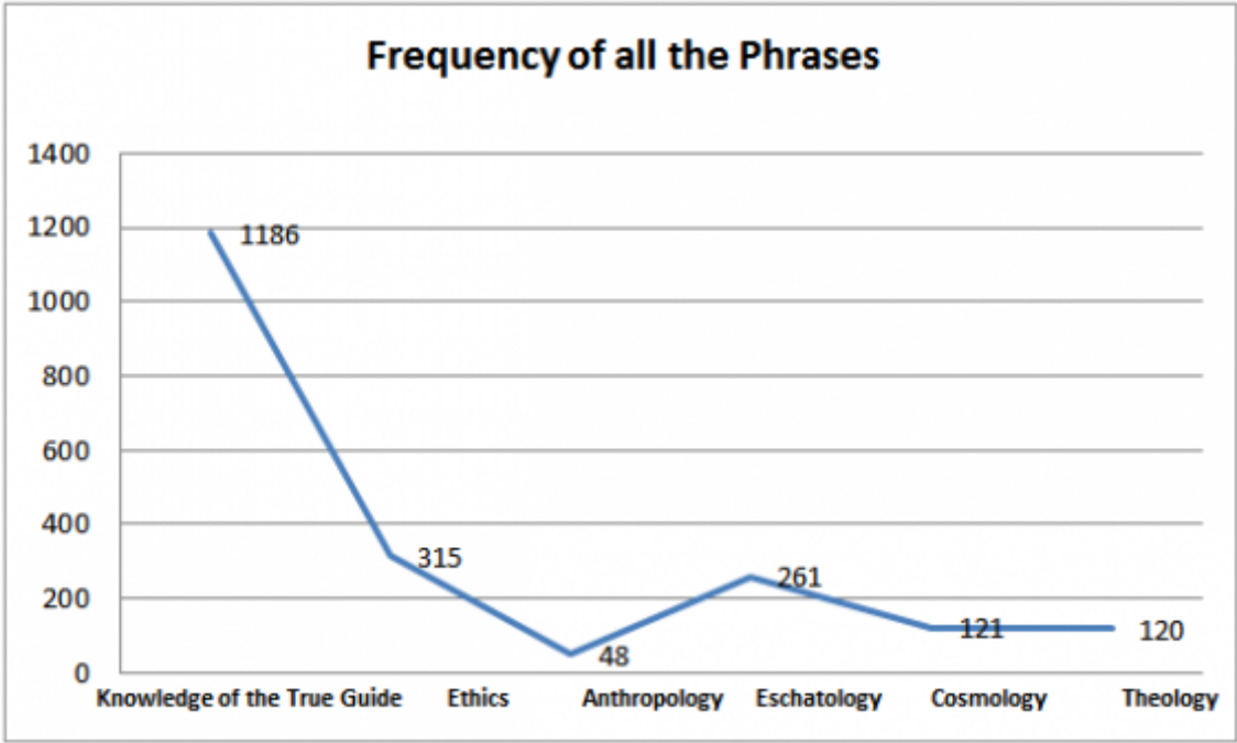
Figure 2: Conclusion 5 .
