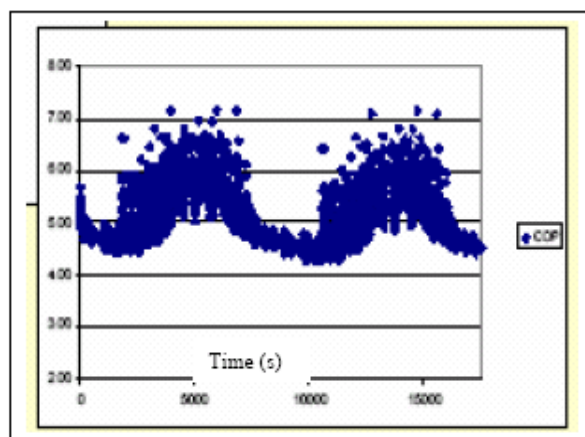
Figure 1 : Coefficient of Performance (COP)
