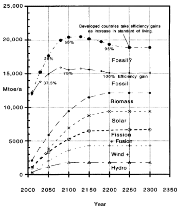
Figure 3 : Total energy uses for 2010-2300 with potential energy sources (added to give total)
