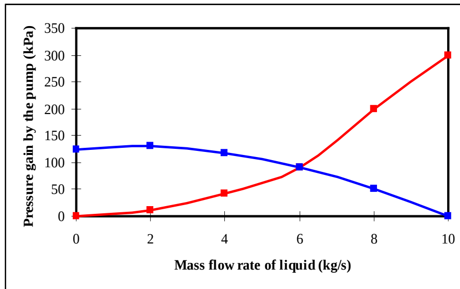
Figure 2 : Balance point (BP) of the pump must coincide with the best efficiency point (BEP)
